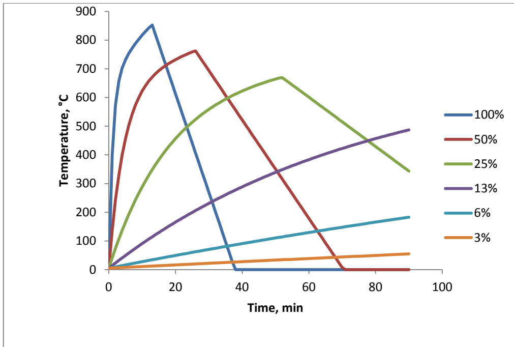
Figure 10: The influence of reducing ventilation on temperature, FLED 400 MJ/m 2
