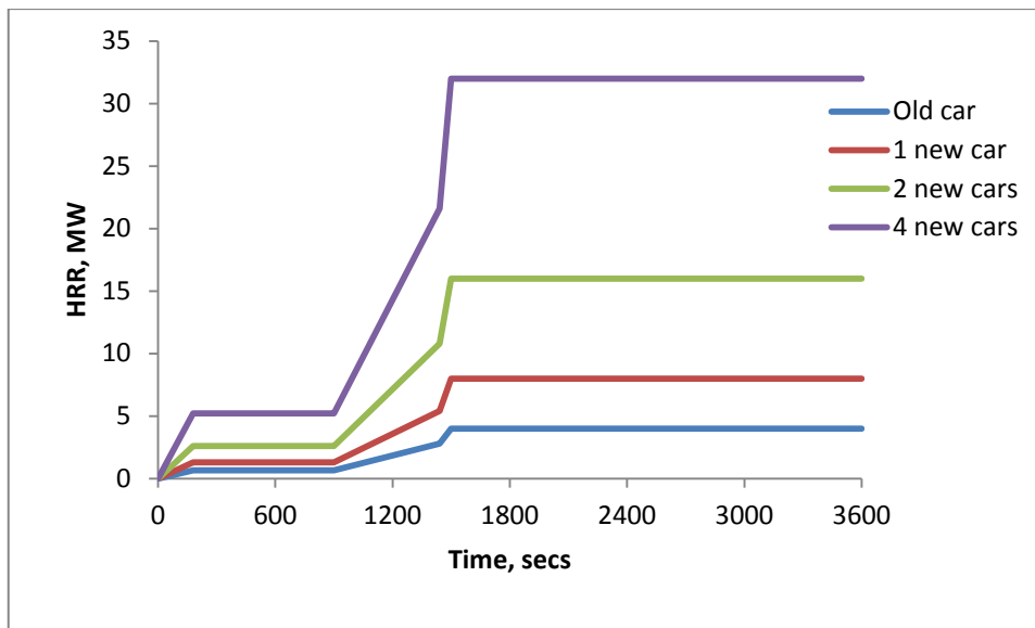
Figure 16: HRR curves for multiple car fires
