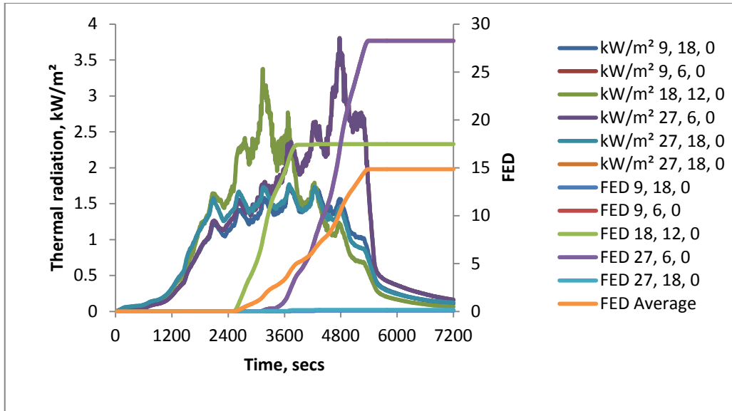
Figure 32: Thermal radiation and FED_{rad} (thermal) for old cars in a closed car park – one x 4 x 3 m (h) door
