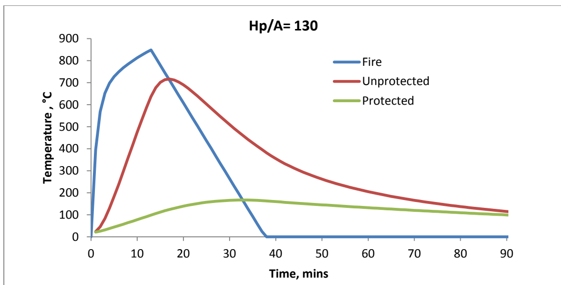
Figure 13: Temperatures reached in steel member for 400 \text{ MJ/m}^2 FLED and fully ventilated fire
