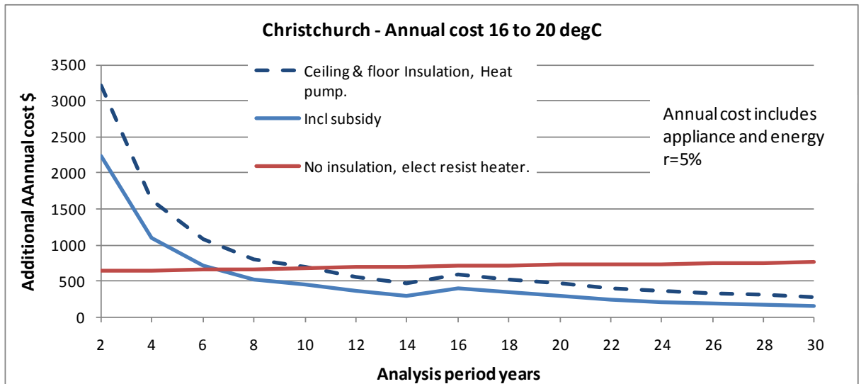
Figure 10. Energy and appliance costs – Christchurch
