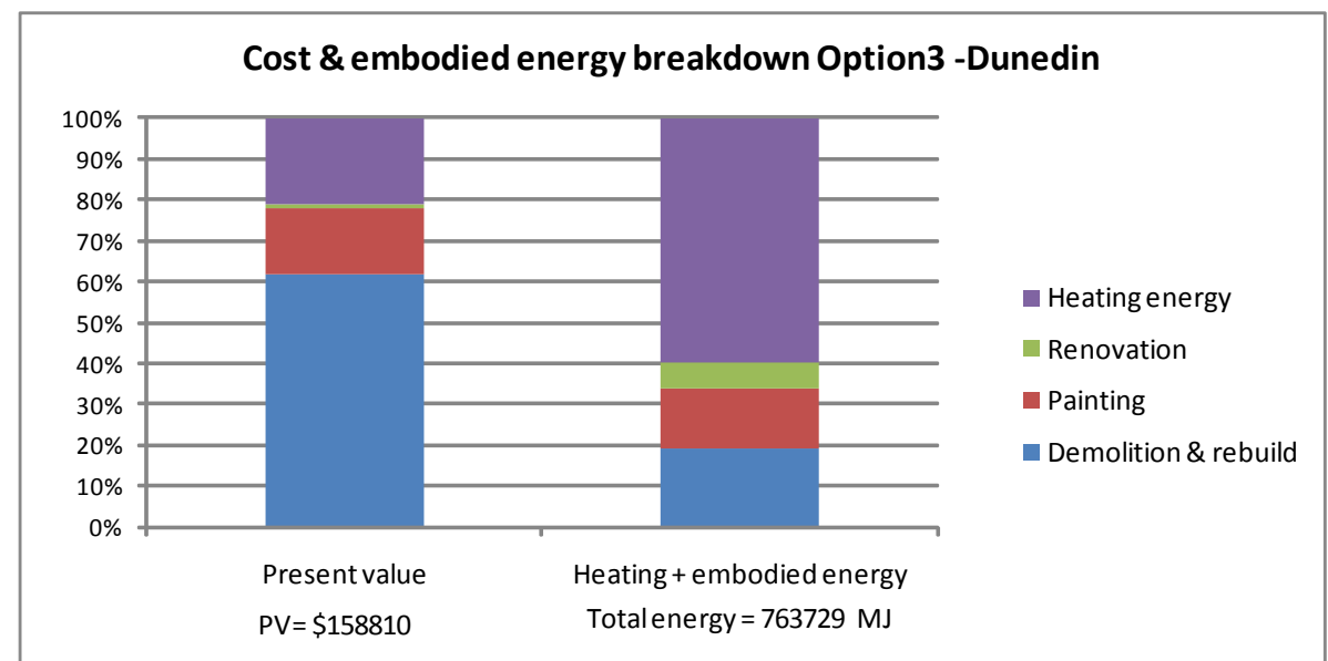
Figure 4. Main work components by cost and energy – Dunedin
