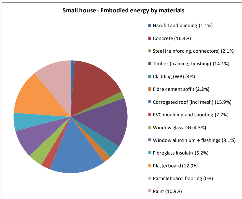
Figure 13. Small house materials embodied energy
