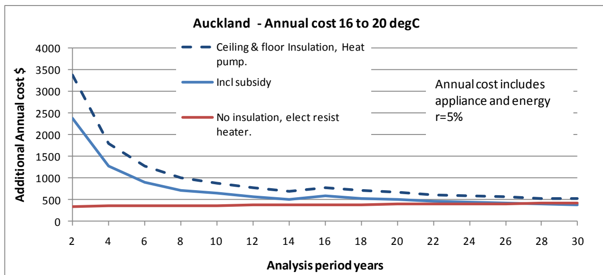
Figure 8. Energy and appliance costs – Auckland
