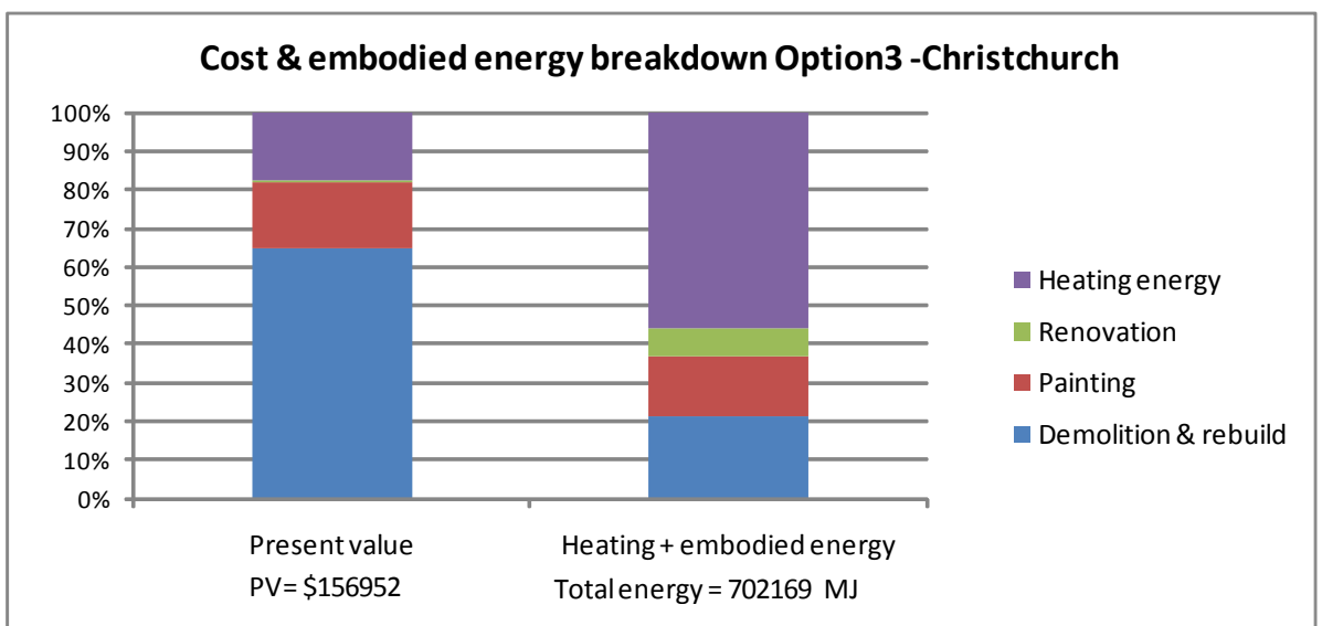
Figure 3. Main work components by cost and energy – Christchurch
