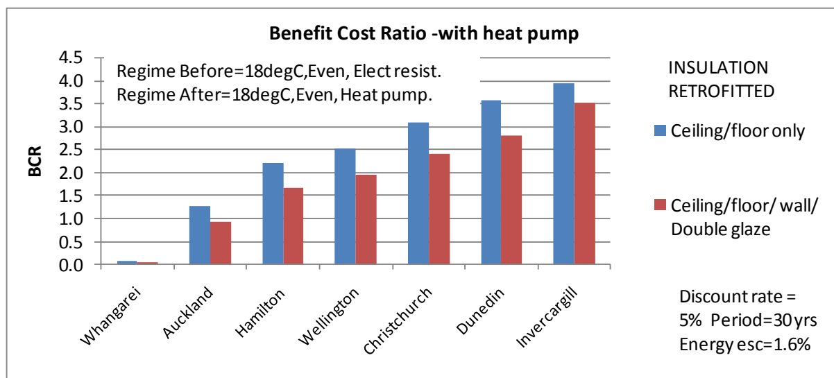
Figure 6. Insulation BCRs – same heating regime before and after, but heat pump retrofit
