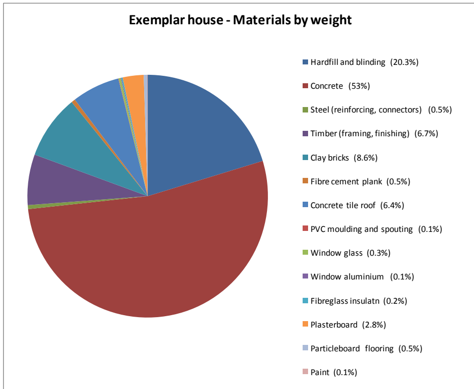
Figure 14. Exemplar House materials by weight
