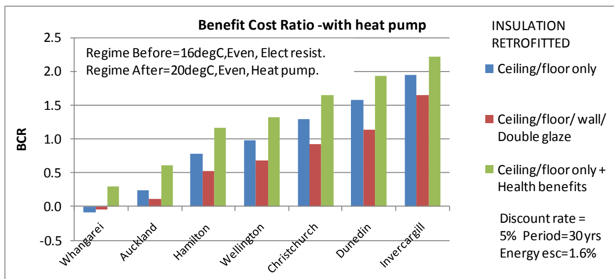
Figure 7. Insulation BCRs – higher temperatures after retrofit, including heat pump retrofit
