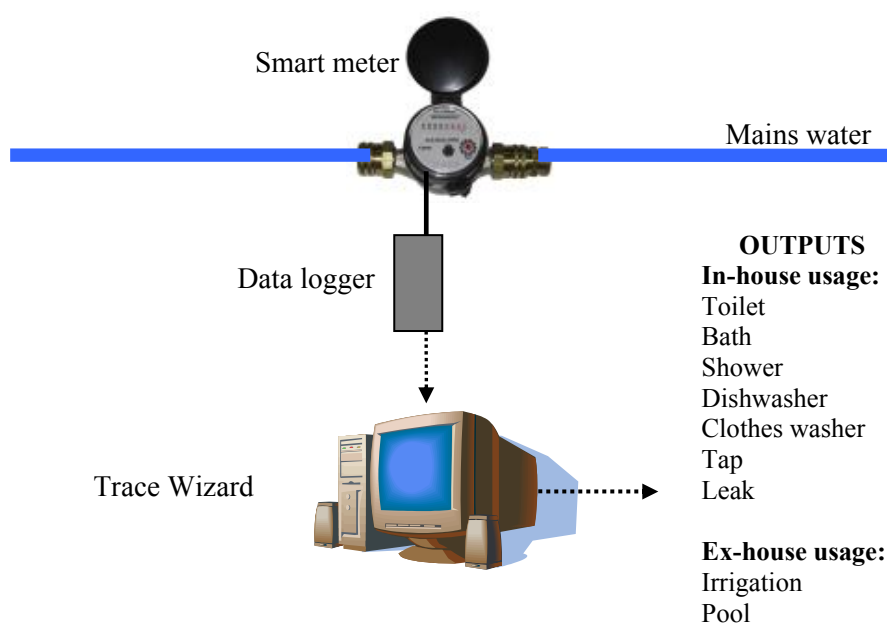
Figure 4: Metering arrangement
