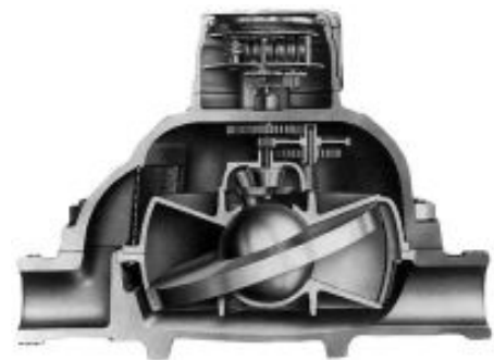
Figure 7: Nutating disk meter (Source: AMS Instrumentation & Calibration Pty Ltd)
