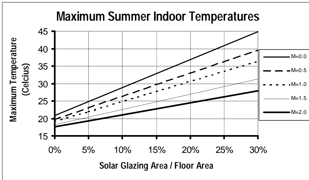
Figure 6. Maximum summer indoor temperature by solar glazing ratio and thermal mass level.
