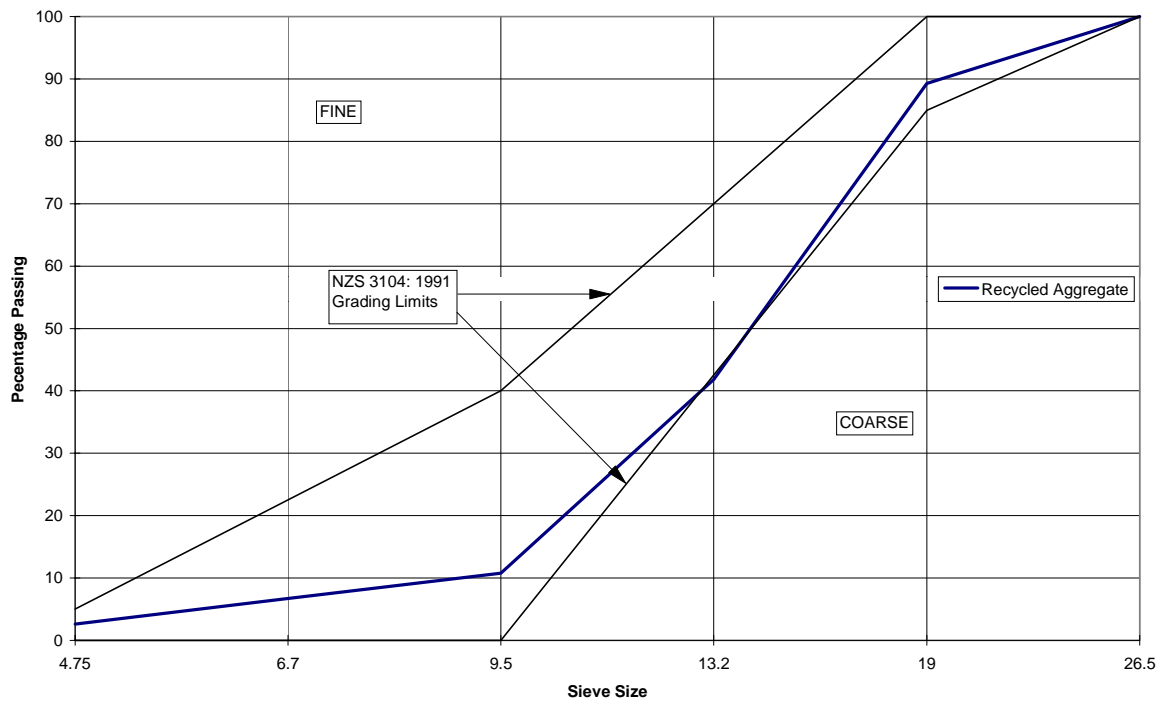
Figure 2. Coarse aggregate grading curve with envelope from NZS 3104 (SANZ 1991).
