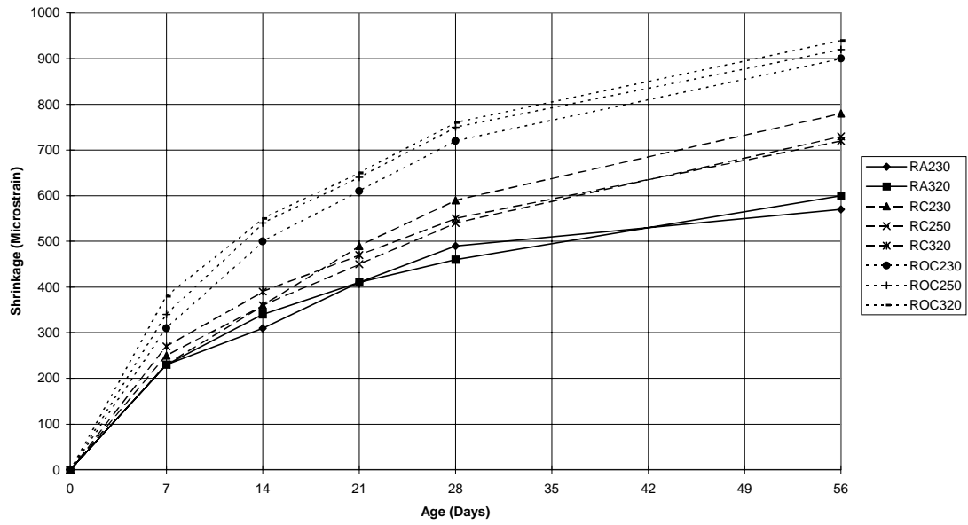
Figure 1. Drying shrinkage of all concretes tested.
