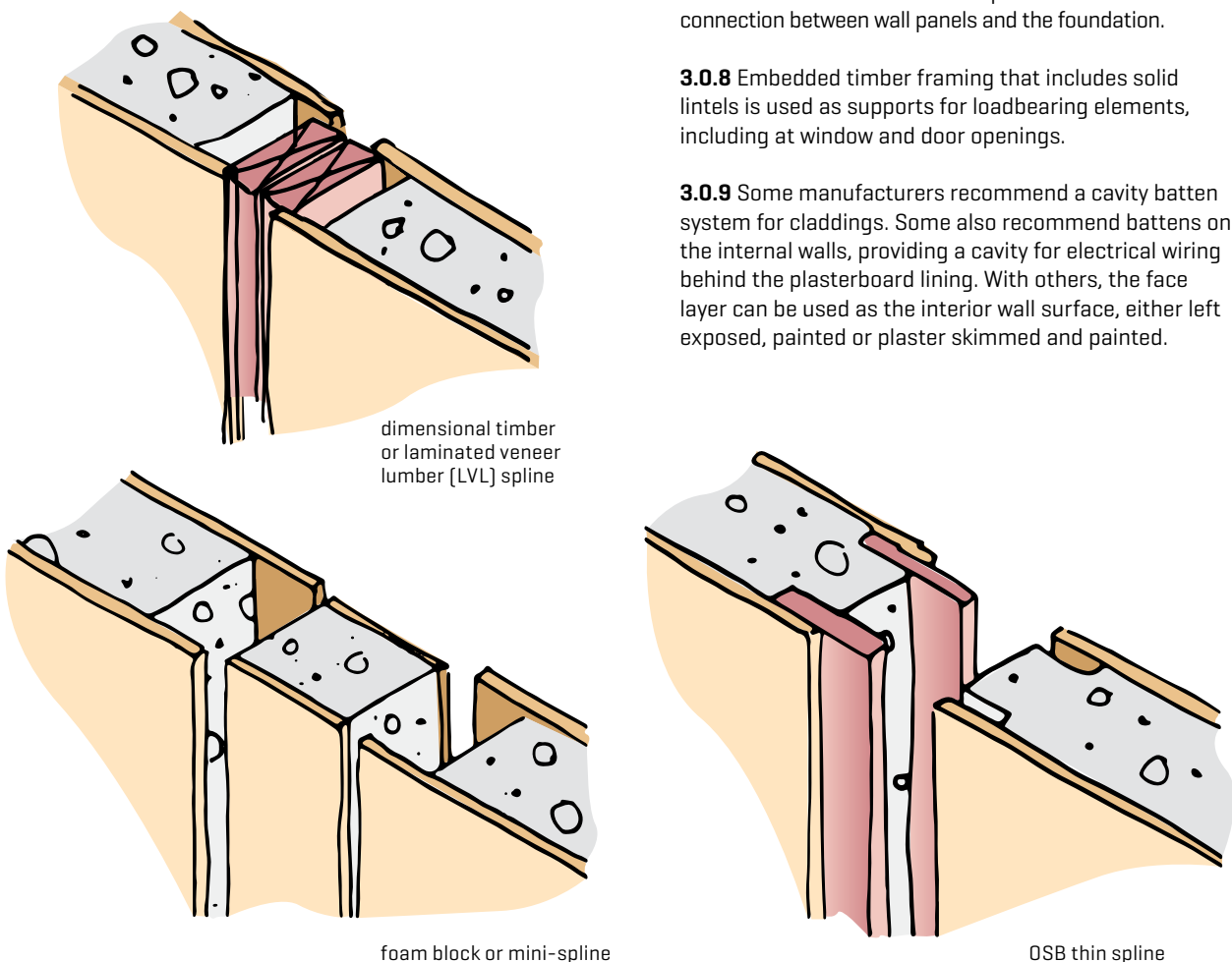
Figure 2. Examples of connections between SIPs.
