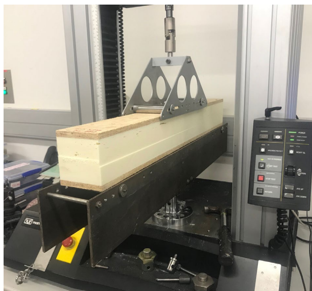
A typical SIP sample in a four-point flexure test set-up.
