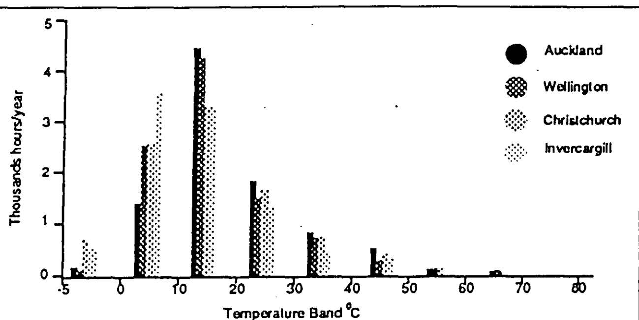
Figure 1: Sol-air temperature frequency distribution for black roofs.
