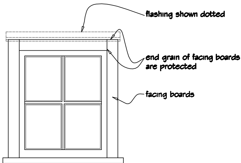
Timber Window Elevation
