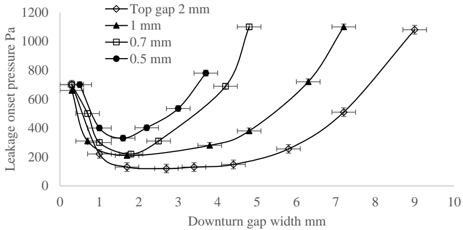
Figure 9. Leakage onset pressures for a 35 mm flashing with a kick-out leg as a function of downturn gap ( w ) and top gap ( t ) dimensions.
