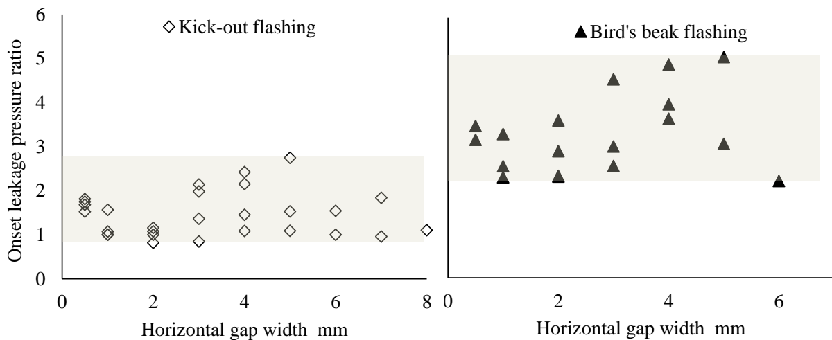
Figure 6. Onset leakage pressure ratios for kick-out and bird's beak flashings compared with a plain-ended downturned flashing.
