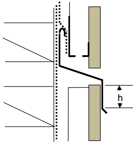
General inter-storey junction
