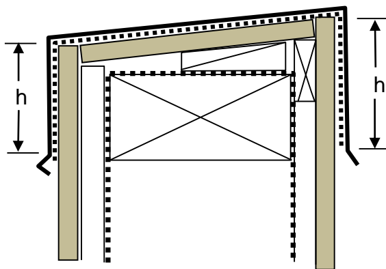
Parapet and enclosed balustrade
