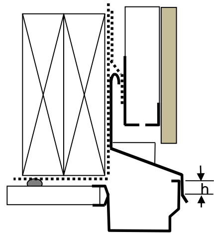
Window head flashing
