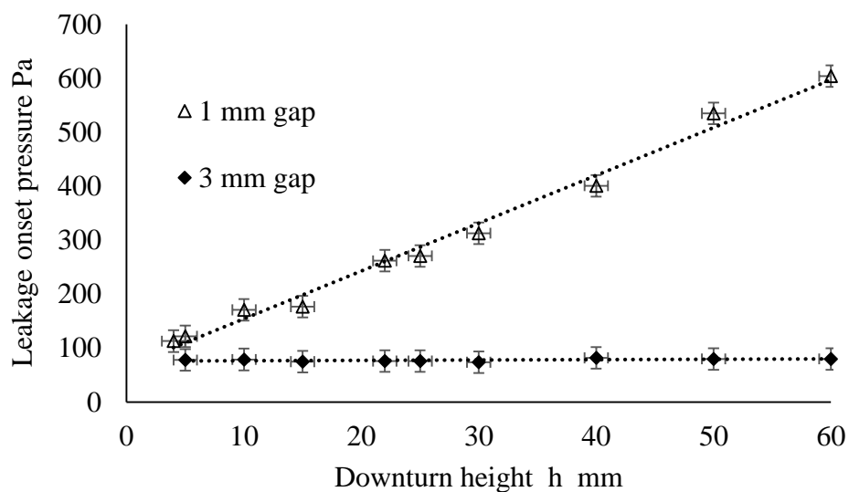
Figure 5. Leakage onset pressures as a function of downturn height ( h ) for a 35 mm downturned flashing with a kick-out and two values of gap width ( w ).
