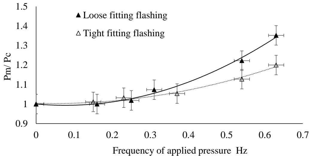
Figure 13. Ratio of measured onset leakage pressure ( P_m ) and the calculated onset leakage pressure ( P_c ) plotted against the frequency of applied air pressure.
