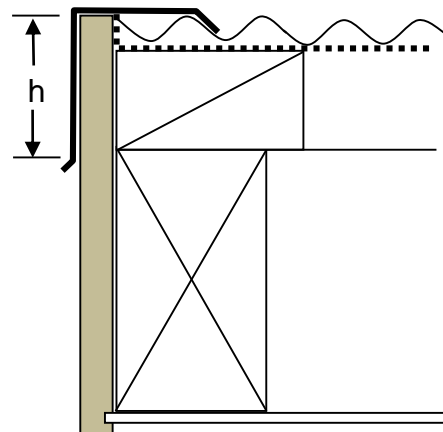
Figure 1. Examples of flashing downturns over cladding components taken from E2/AS1.
