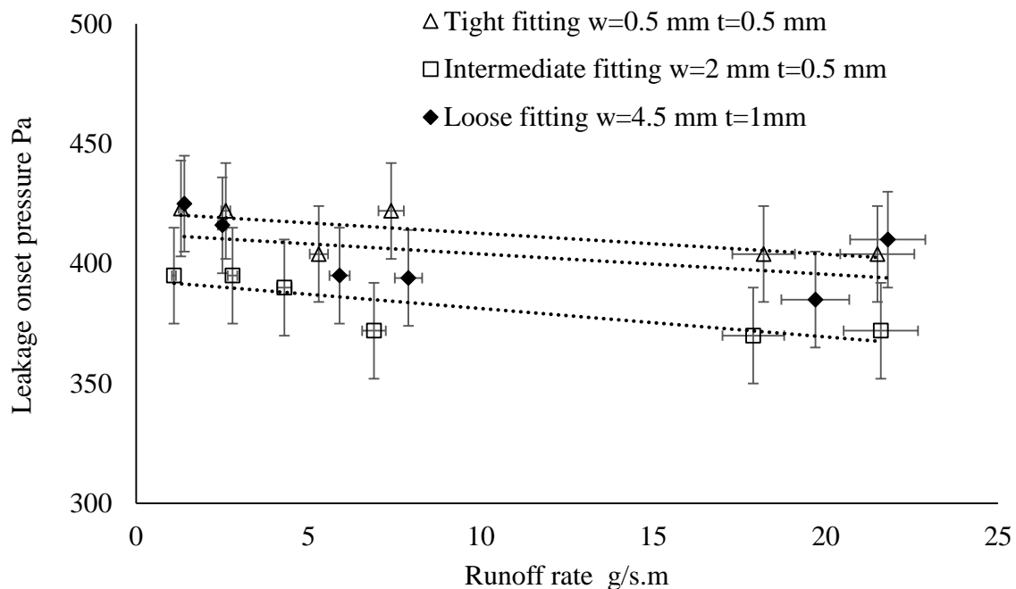
Figure 4. Leakage onset pressures as a function of run-off rate for a 35 mm flashing downturn and a kick-out end.
