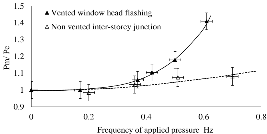
Figure 14. Ratio of measured onset leakage pressure ( P_m ) and the calculated onset leakage pressure ( P_c ) plotted against the frequency of applied air pressure. This data is for a window head flashing and a non-vented inter-storey junction.
