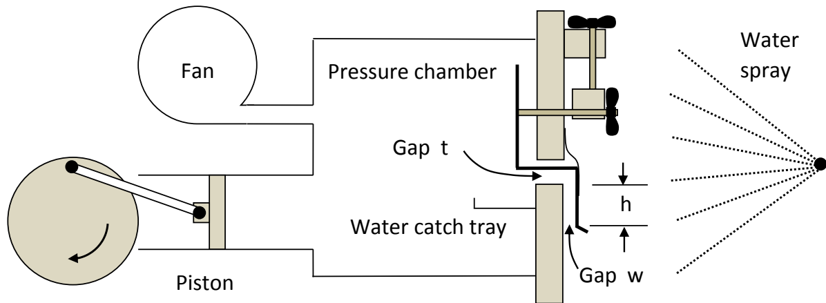
Figure 3. Equipment for adjusting flashing and measuring water leakage rates through a downturned flashing.
