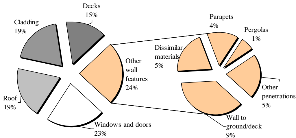
Figure 2. Location of water entry in New Zealand leaking buildings.
