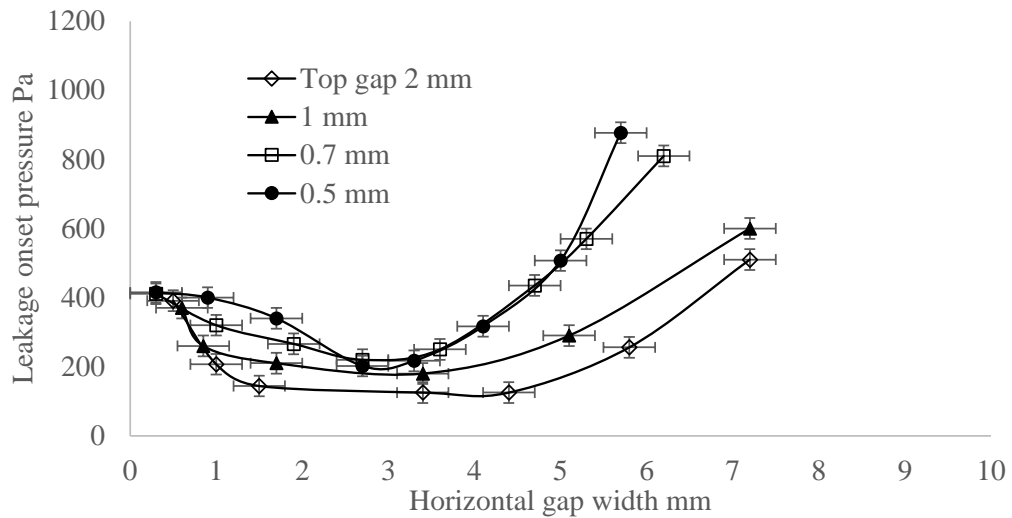
Figure 7. Leakage onset pressures for a 35 mm flashing with a plain leg as a function of downturn gap ( w ) and top gap ( t ) dimensions.
