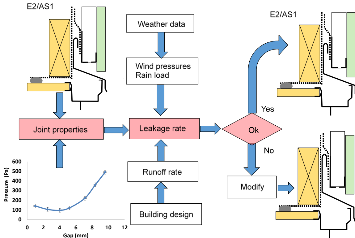
Figure 15. Schematic of the process for modifying a junction detail to take account of high wind and rain loads on a façade.
