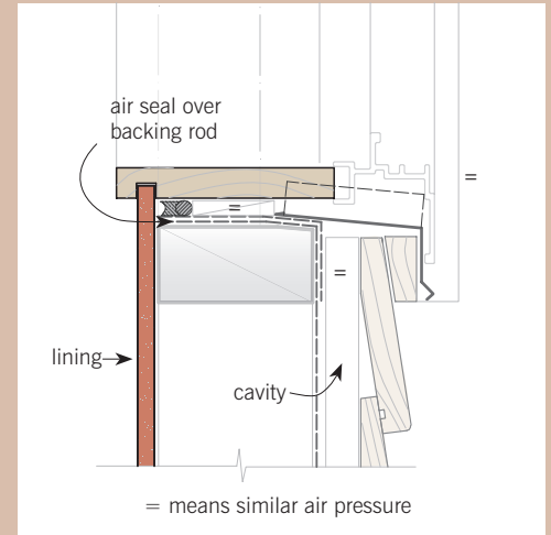
Figure 2: The same window, but with an air seal and backing rod.
