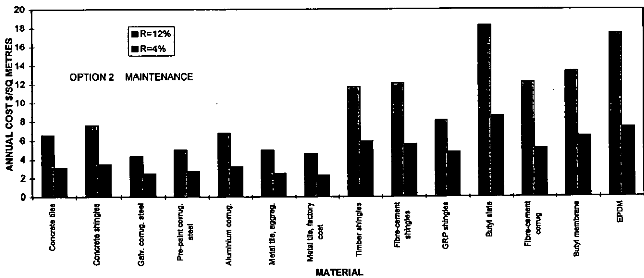
ROOF CLADDING ANNUAL COST v DISCOUNT RATE MODERATE ENVIRONMENT
