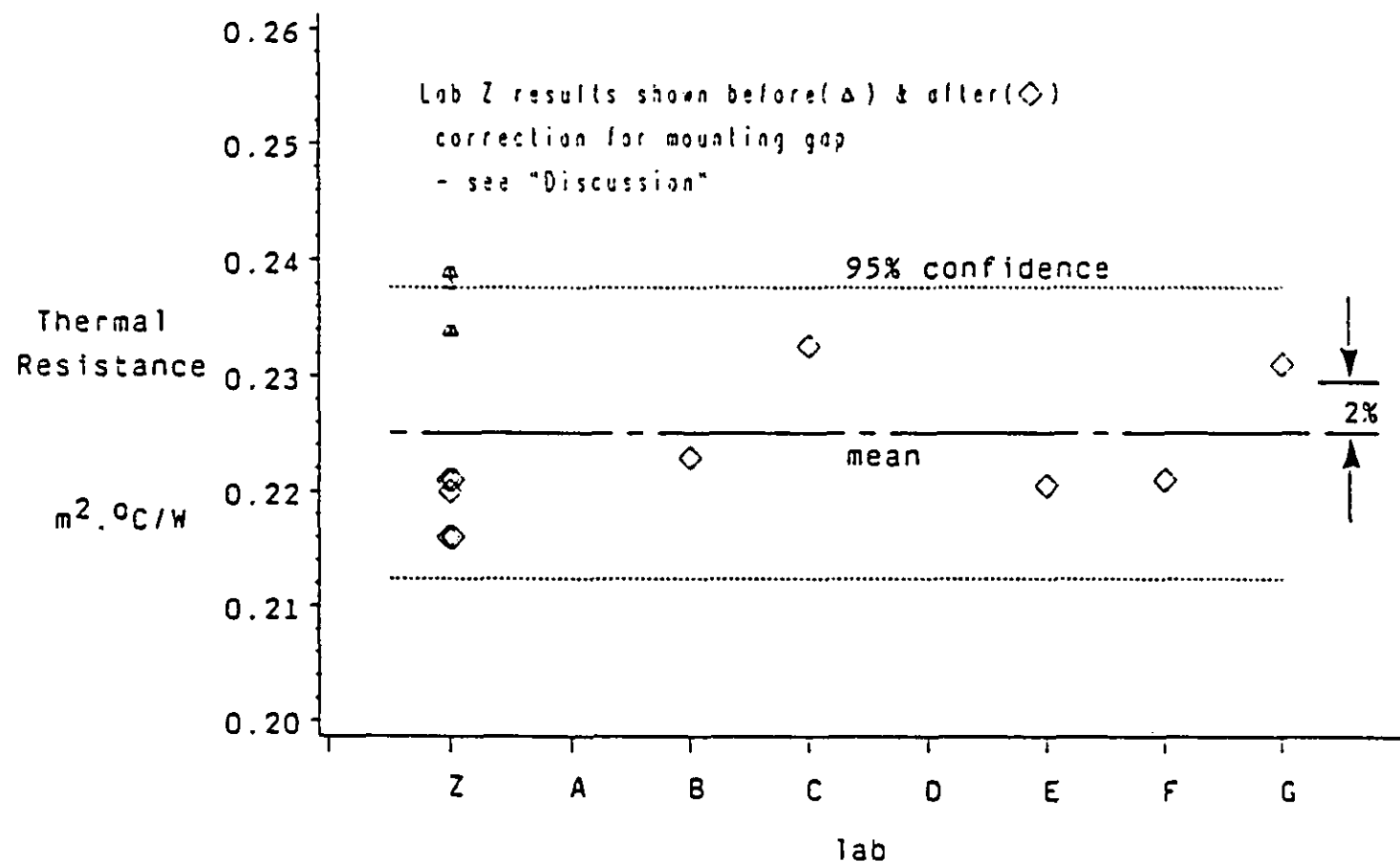
FIGURE 4. COMPARISON OF ALL RESULTS - Mineral Fibre Board
