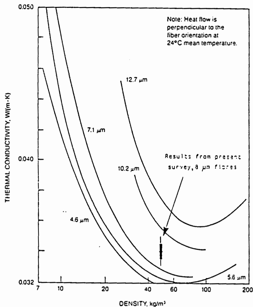
Apparent Thermal Conductivity of Glass Fibers (Lotz 1969)
